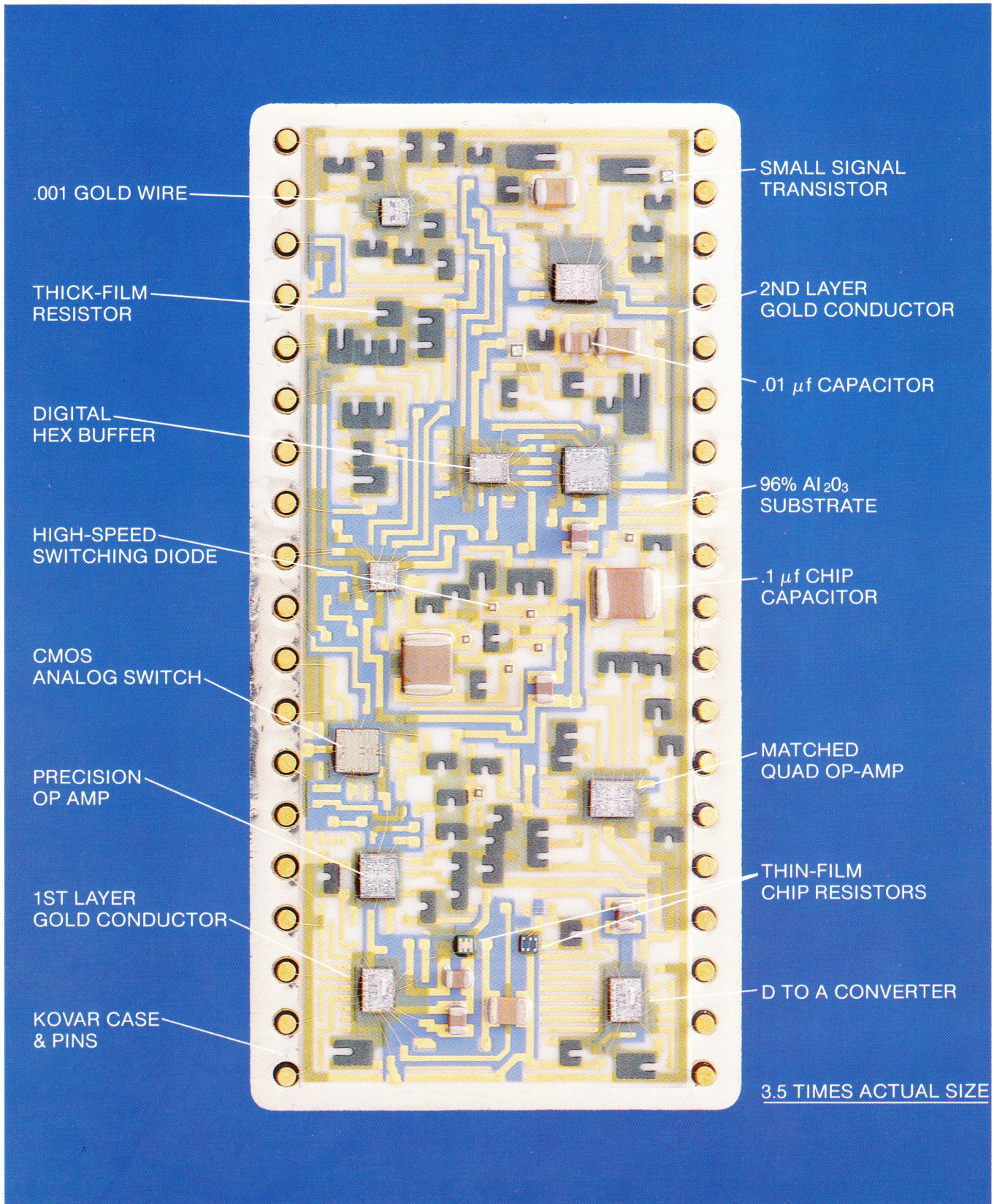
Thick-film hybrid circuits can incorporate a variety of components and technologies.
